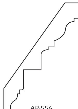
AP-556 3/4" x 5-1/4"
