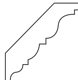
AP-537 3/4" x 3-3/4"
