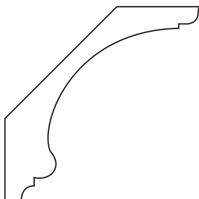
AP-563 1-1/2" x 5-5/8"
