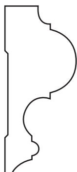
AP-639 1-1/2" x 3-5/8"
