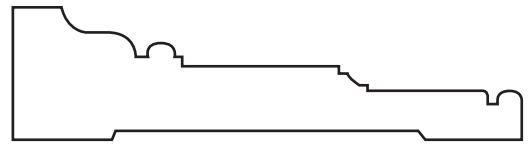
AP-168 1-3/8" x 5-1/4"
